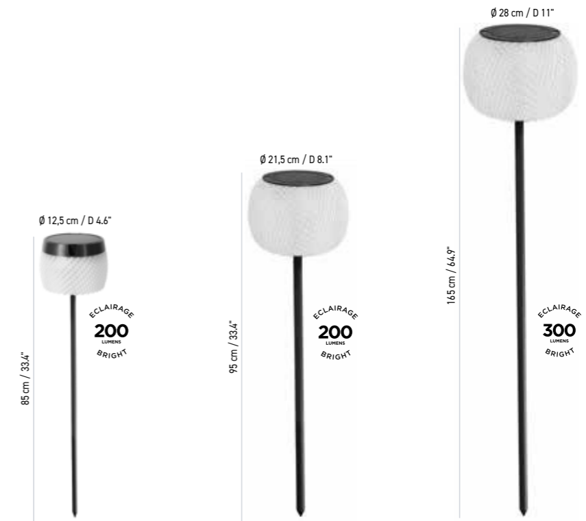
TORCHE LOLIE SMALL À PLANTER LOLIE SMALL GARDEN TORCH TO PLANT
