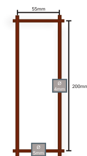
Panneau EXPERT 55 Medium
