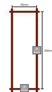
Panneau EXPERT 55 Premium
