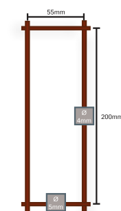
Panneau EXPERT 656 Premium
